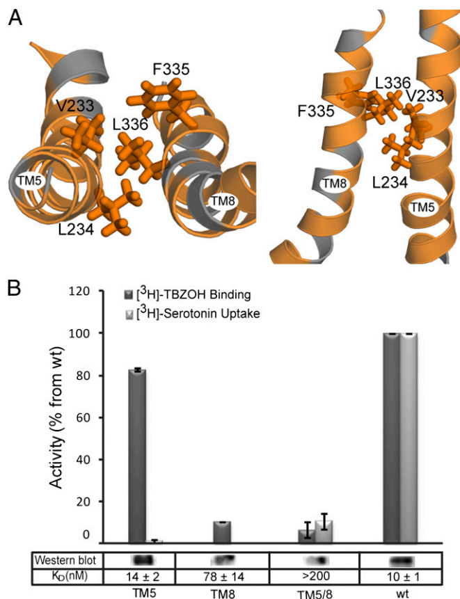
Fig. 6. Predicted hydrophobic interactions between TM5 and TM8. (A) Close-up of TMs 5 and 8 in the cytoplasm-facing model of rVMAT2 viewed as in Fig. 2A (Left) and along the plane of the membrane (Right) with the cytoplasm toward the bottom. Hydrophobic residues (Ala, Gly, Val, Ile, Leu, Phe, Met, and Trp) are colored orange. Side chains of L336, F335, L234, and V233 are shown as sticks. (B) [ 3 H]-TBZOH binding to HEK239 permeabilized cells, [ 3 H]-serotonin transport for V233A/L234A (TM5), F335A/L336 (TM8), and the quadruple mutant V233A/L234A/F335A/L336 (TM5/8), and Western blot relative to wild-type rVMAT2. Results presented are from duplicate experiments; error bars indicate SE. Experiments were repeated at least twice.
